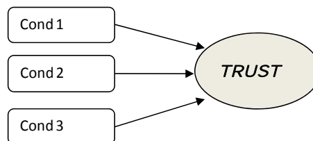
Figure 1: Variance relations
